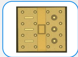
Flip-Chips
