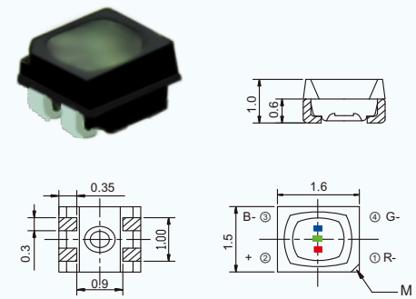
FM-B1515RGBA-HG 1.6×1.5×1.0
