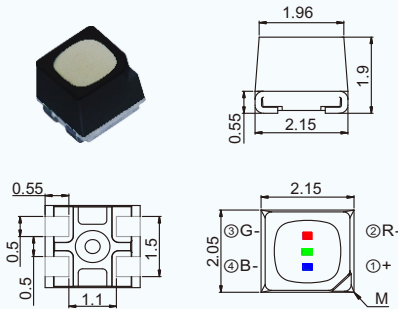
FM-Z1921RGBA-SH 2.15×2.05×1.9
