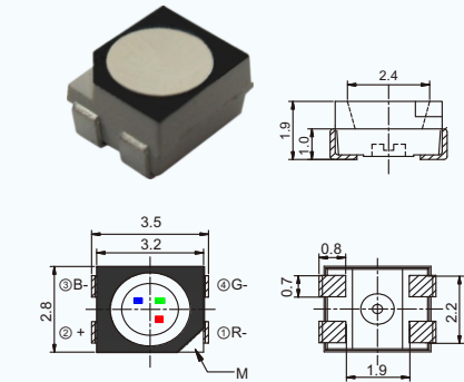
FM-3528RGBA-HF 3.5×2.8×1.9
